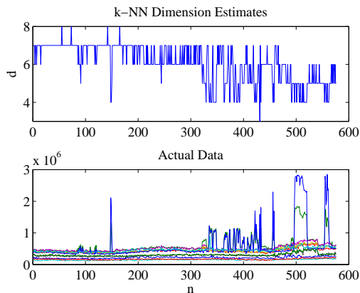
Fig. 4. The k -NN Algorithm applied to network traffic data
