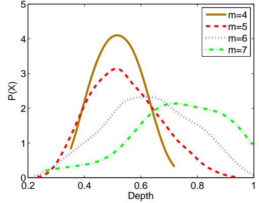
Fig. 2. Analysis of the effect of data depth on local dimension estimation. Points with less depth estimate at a lower dimension, contributing to the overall negative bias.
