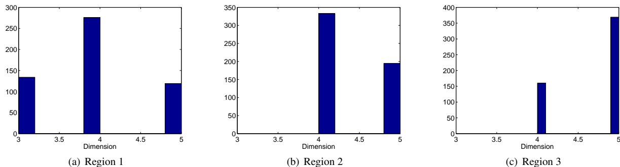
Fig. 6. Dimension estimation can be used for image segmentation by observing the difference in estimates of region complexity
