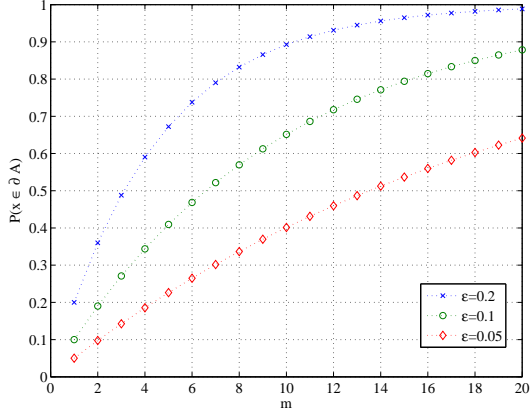
Fig. 1. The probability of randomly selecting a point on the boundary of an m -dimensional hypercube for \epsilon = 0.2 ( \times ), \epsilon = 0.1 ( \circ ), and \epsilon = 0.05 ( \diamond ).
