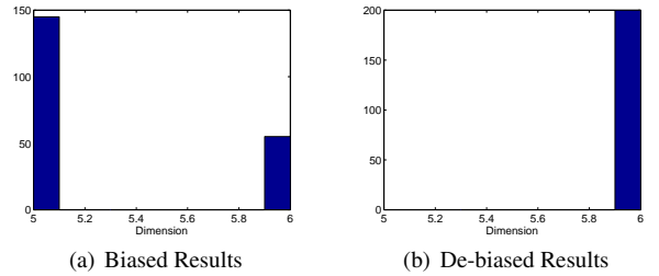
Fig. 3. Developing a de-biased global dimension estimate by averaging over the 50% of points with the greatest depth on the manifold
