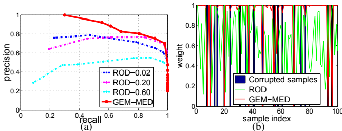
Fig. 2: (a) Recall-precision curve for GEM-MED and RODs on simulated data (corruption rate = 0.2). (b) Illustration of anomaly score \hat{\eta}_n for GEM-MED and ROD-0.2. GEM-MED surpluses ROD in anomaly detection.
